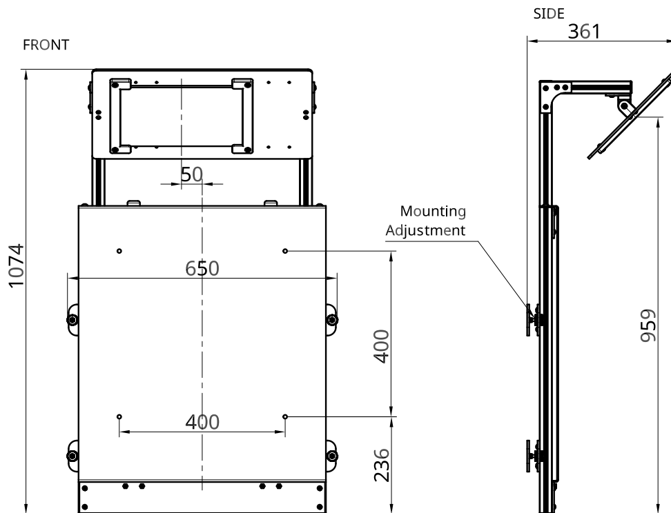
Example Drawing shows VMM-UP for Barco Medea. All Mounts are custom made for the projector
